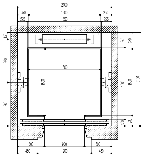
DETAILED SHAFT HOISTWAY & ELEVATOR SPECT.
