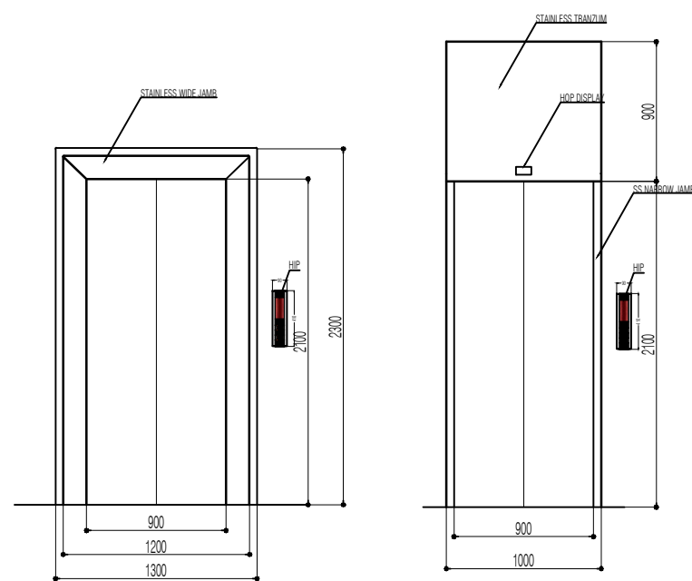
DETAILED I OPENING ENTRANCE PLANN FOR 2FL - 5FL (CENTRE OPENING)
