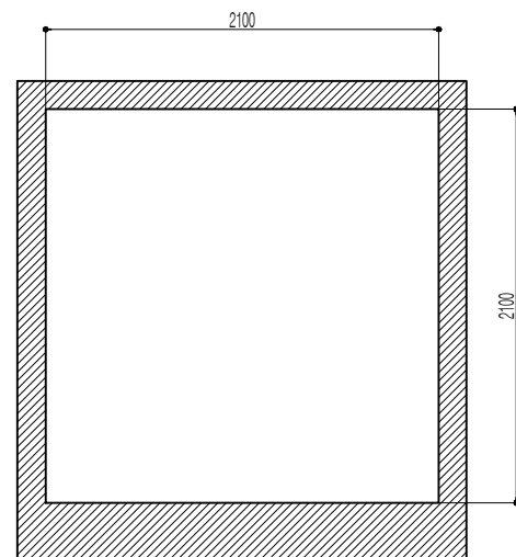
DETAILED SHAFT HOISTWAY & CONSTRUCTION PLANN
