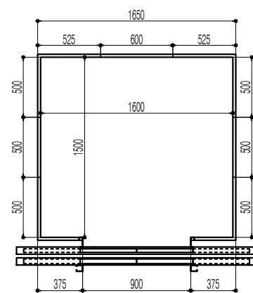
LAY OUT FLOOR & WALL PANEL
