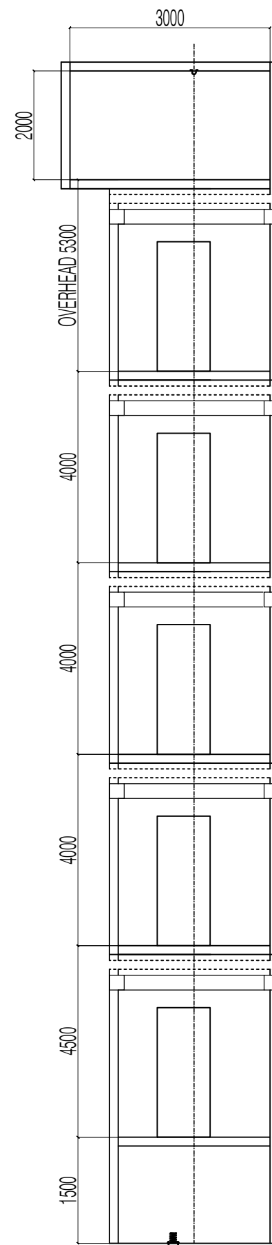
SECTION OF HOISTWAY PLANN FRONT VIEW
