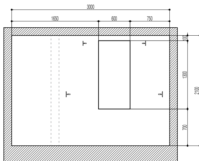
MACHINE ROOM PLANN
